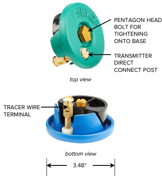
SNAKEPIT ® SINGLE-TERMINAL CAST IRON LID
